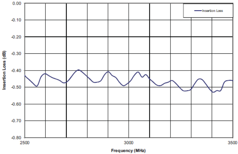
RFLM-252352QC-290 Insertion Loss vs Frequency
