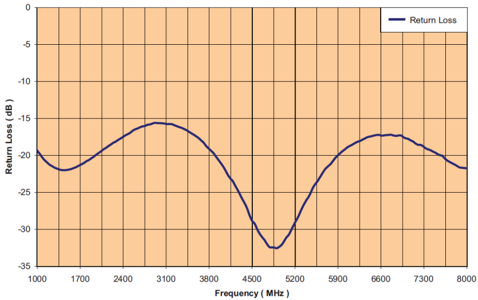
RFLM-202802QC-290 Return Loss vs Frequency
