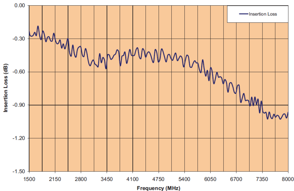
RFLM-202802LC-299 Insertion Loss vs Frequency
