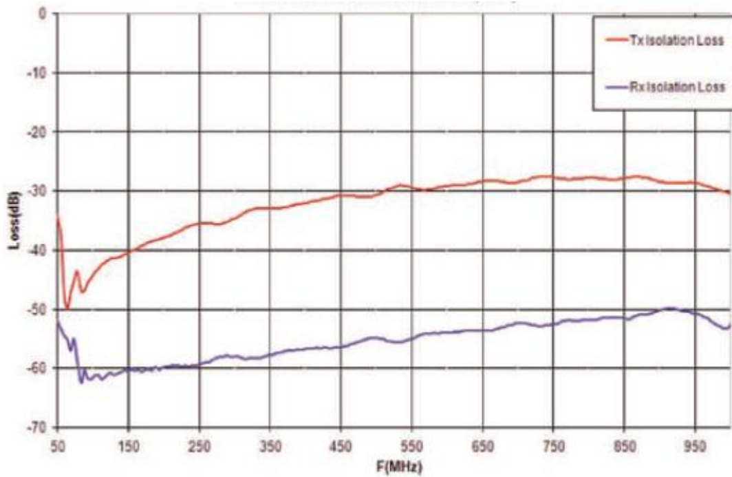
MSW2T-2050-194: Tx and Rx Isolation vs Frequency
